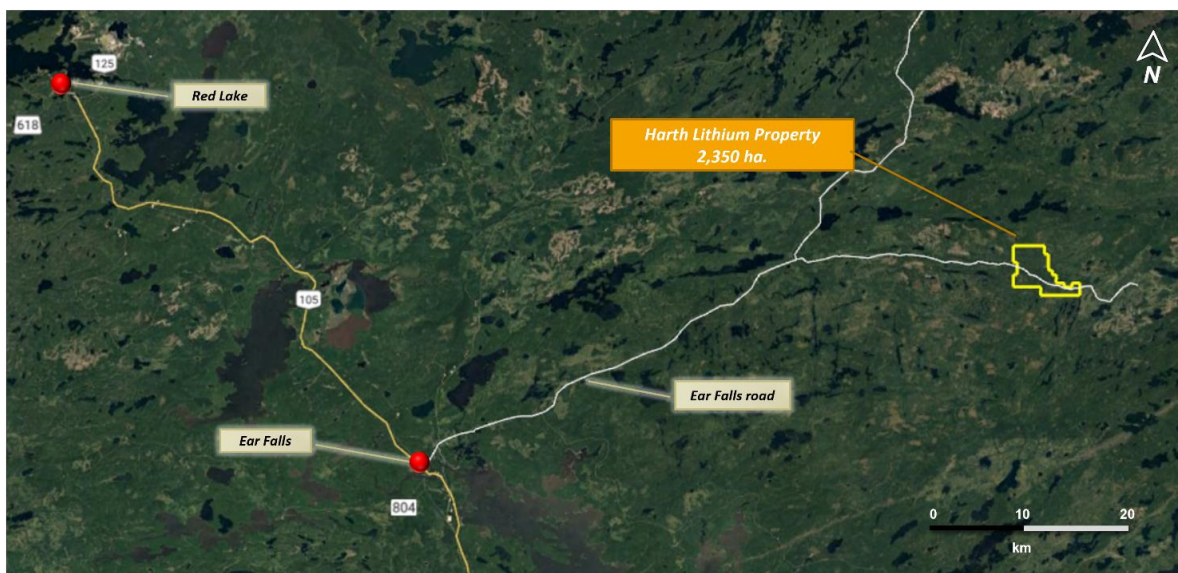
Figure 1. Regional location of the Harth Lithium Property, northwestern Ontario.
